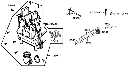
F18 Step BarStandSide
